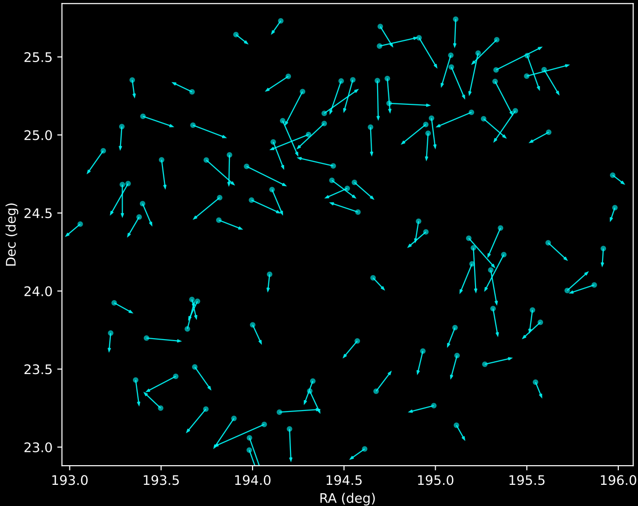
APOGEE DR17 Noise Stream Proper Motion Vectors (n=108)
