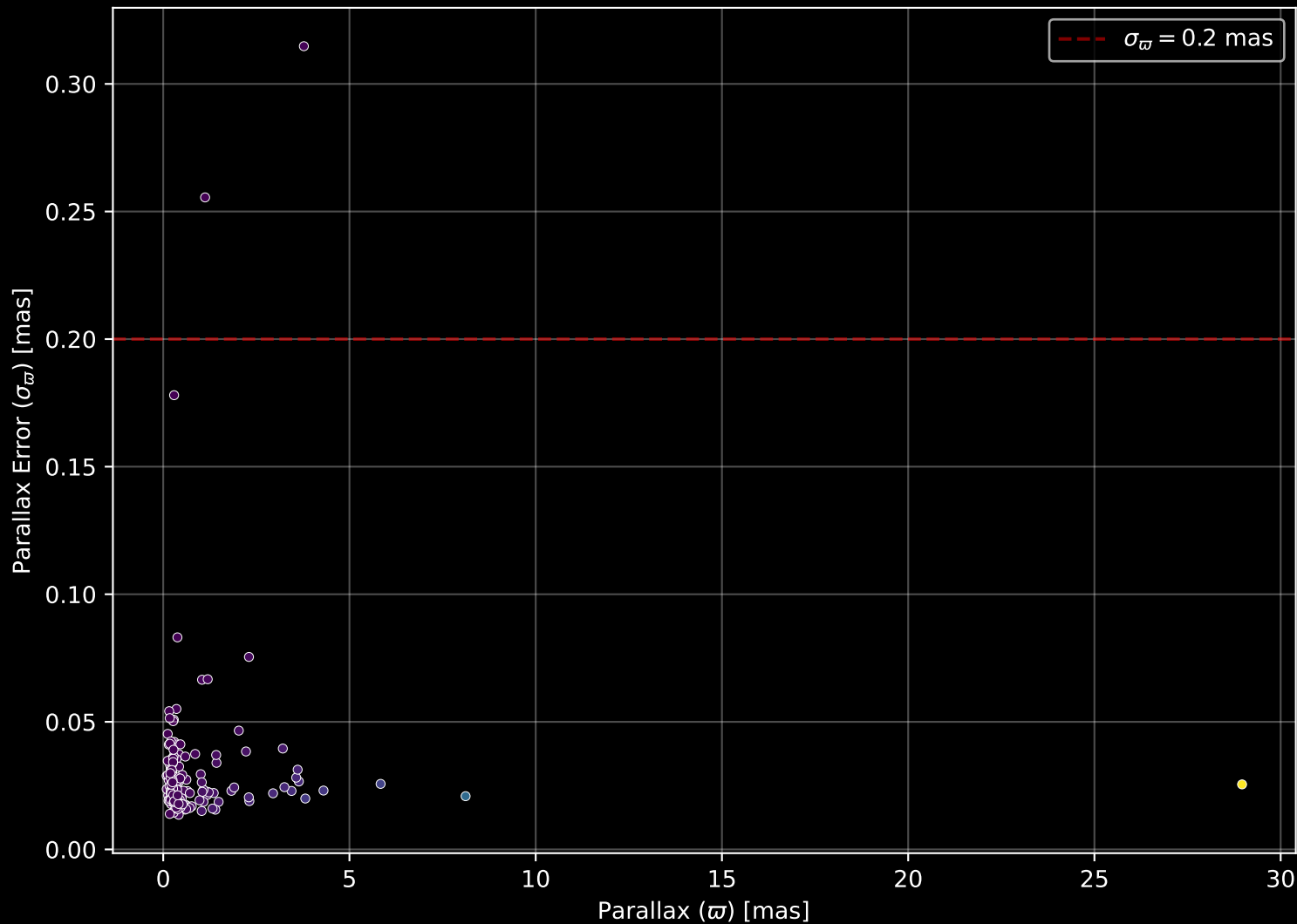
APOGEE DR17 Field: [188+04] Parallax Quality (n= 196)
