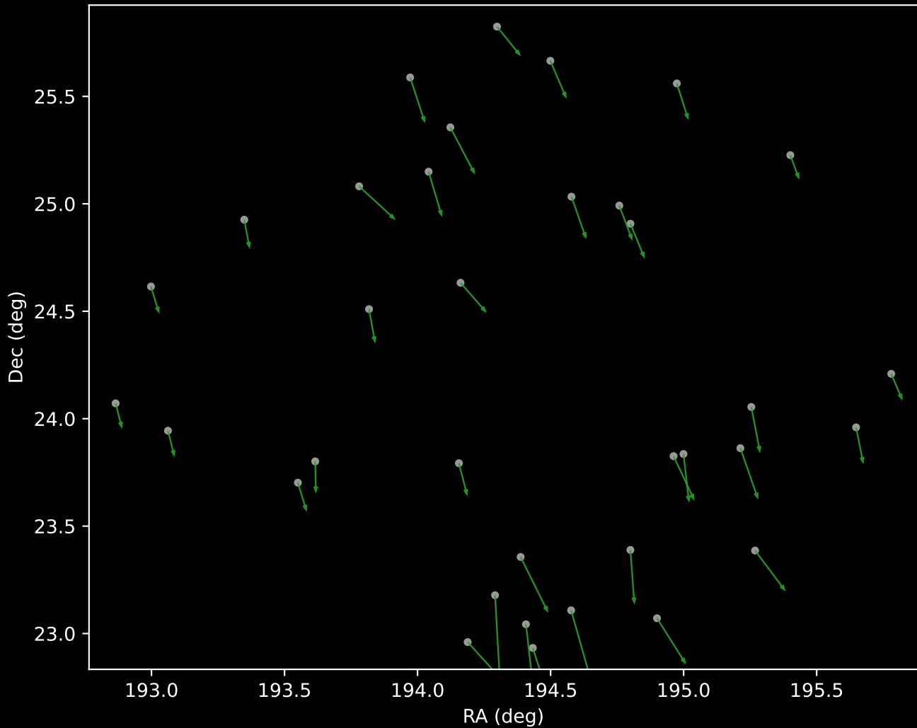
APOGEE DR17 Cluster 4 Proper Motion Vectors (n=35)
