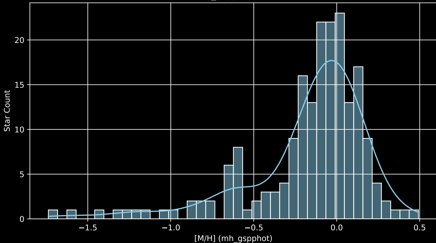
APOGEE DR17 Field: [188+04 [M/H] (mh_gspphot) (n= 195)
