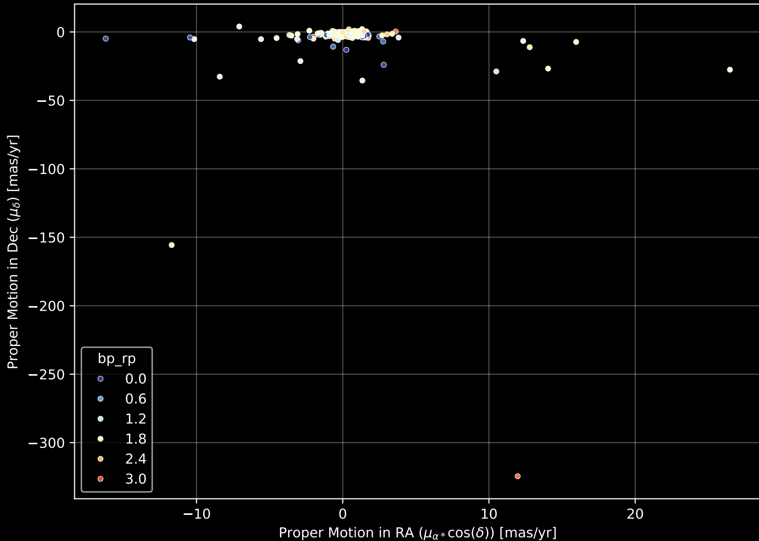
APOGEE DR17 Field: [188+04] Proper Motion Diagram (n= 196)
