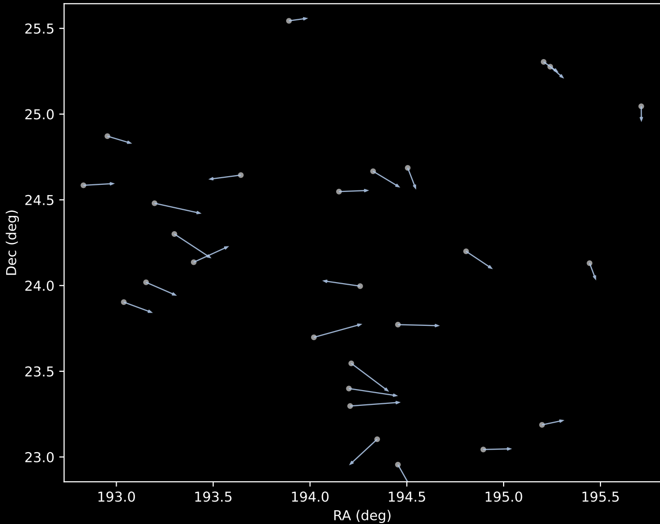
APOGEE DR17 Cluster 1 Proper Motion Vectors (n=27)
