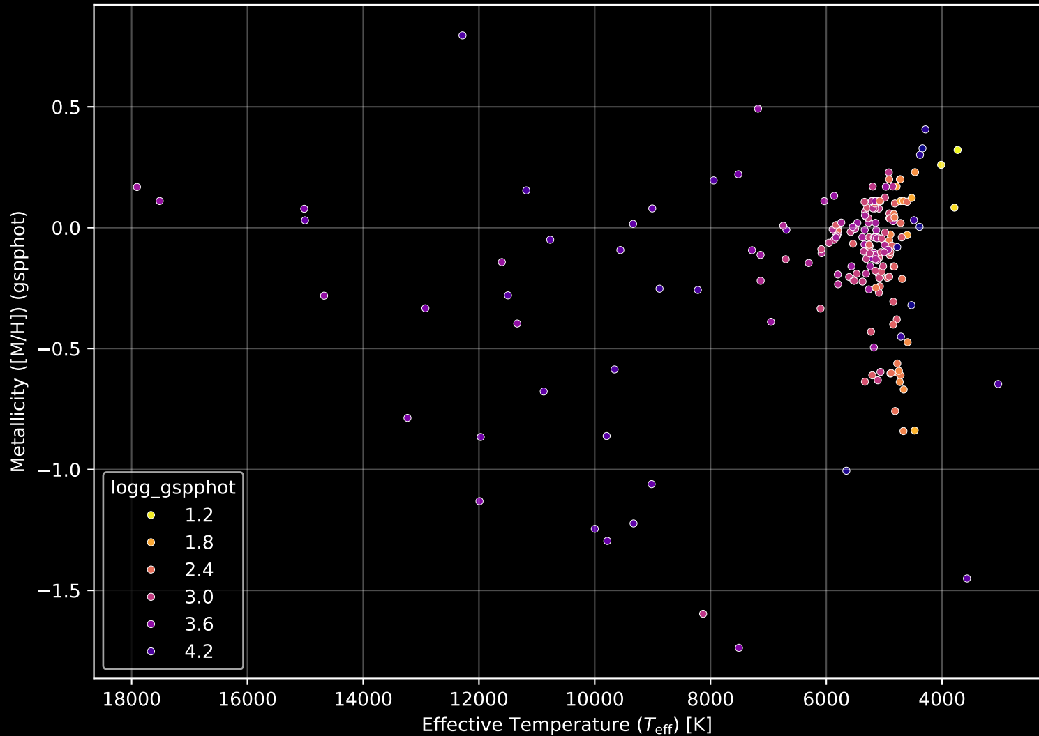
APOGEE DR17 Field: [188+04] Stellar Population Parameters (n= 196)
