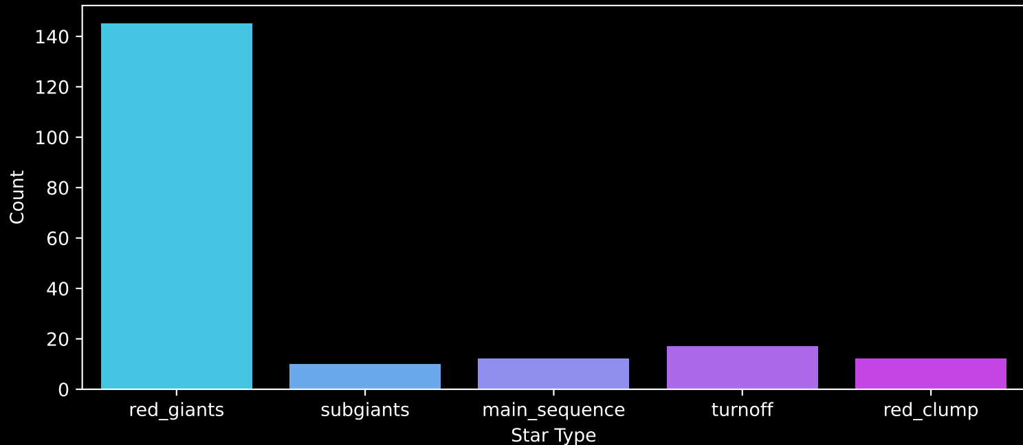
APOGEE DR17 Field: [188+04] Count plot of Star Type
