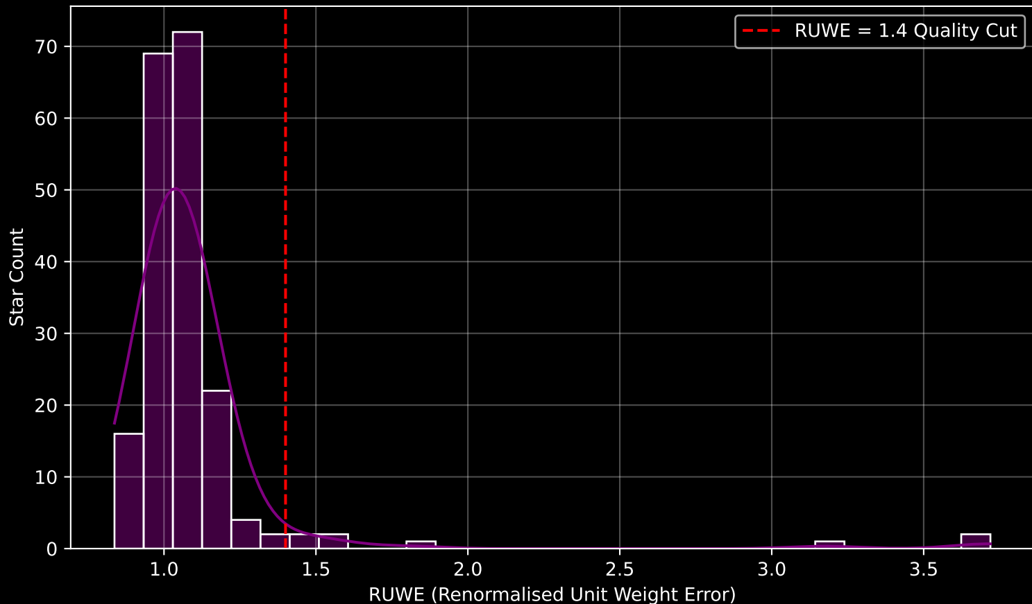
GAPOGEE DR17 Field [188+04] RUWE Distribution (n= 193)
